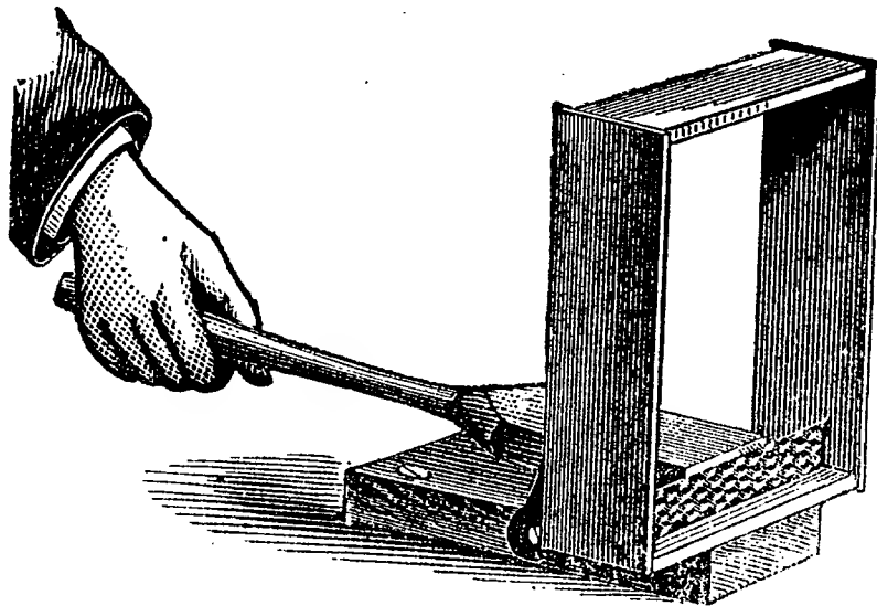
Parker Foundation Fastener.
